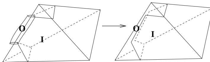
FIGURE 10. Non-parallel normal triangles
