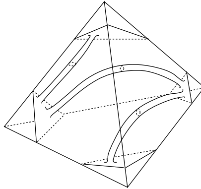
FIGURE 39. There are no more than three tubes
