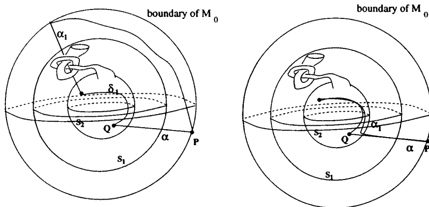
FIGURE 44. Isotoping \alpha_i to \alpha
